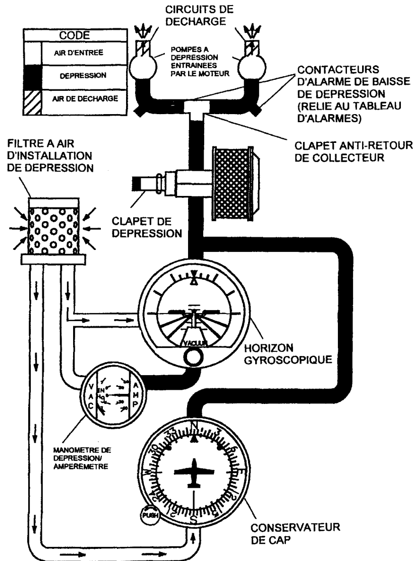
Figure 7-9. Circuit hydraulique
